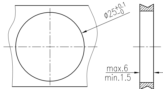
面板安装开孔图I Panel cut out I
