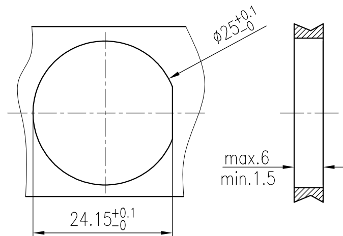
面板安装开孔图II Panel cut out II
