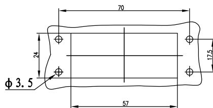
面板开孔图 Panel cut out
