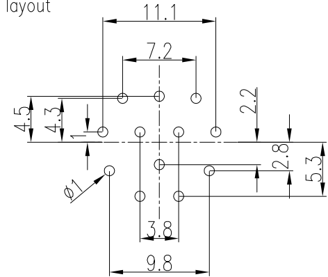
PCB孔细节 PCB layout
