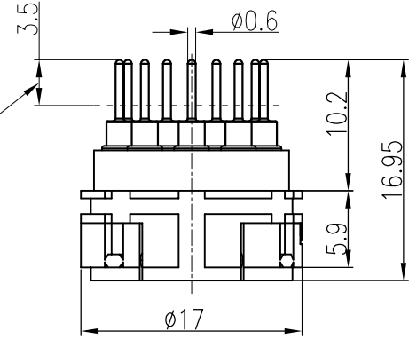
插针插接长度 reference to bulkhead mounted housing
