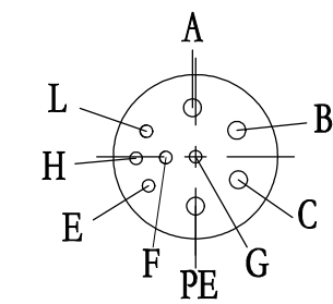
针位排布图 Contact arrangement
