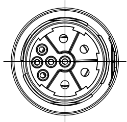
针位排布图 Contact arrangement
