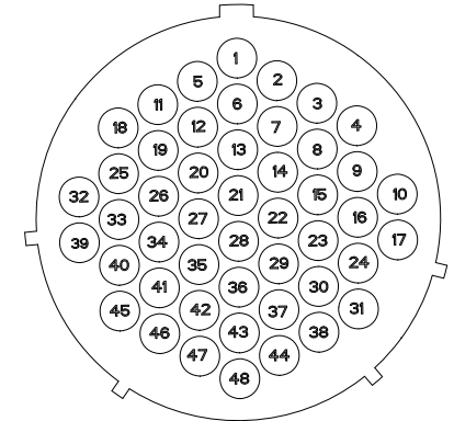
针位排布图 Contact arrangement
