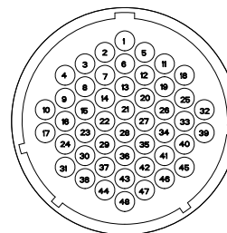
针位排布图 Contact arrangement
