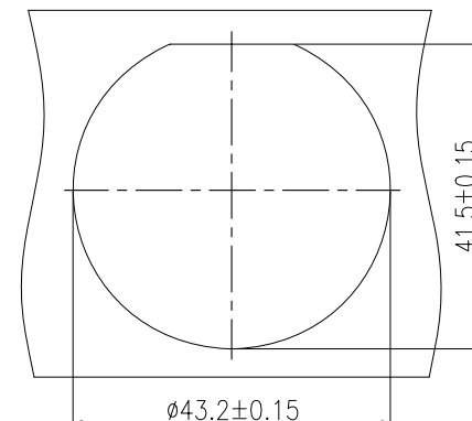
面板安装尺寸 Panel Cut-out
