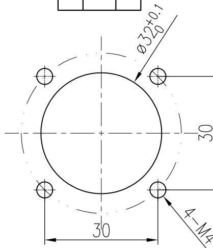
面板开孔图 Panel cut out
