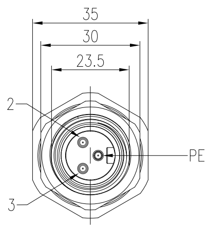
针位排布图 Contact arrangement
