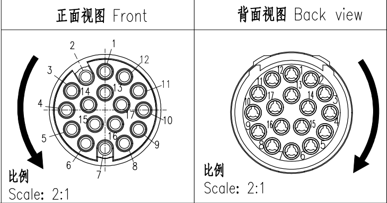
针位排布图 Contact arrangement
