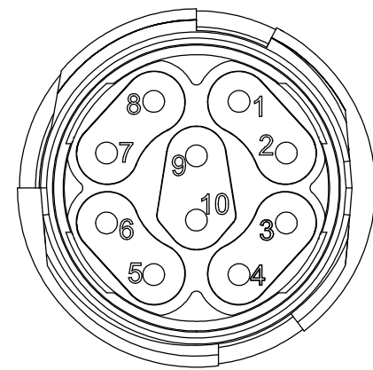
针位排布图 Contact arrangement
