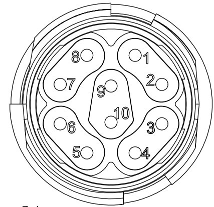
针位排布图 Contact arrangement
