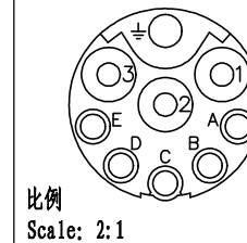
面板安装开孔图 Panel cut out
