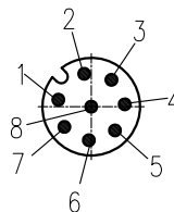
Contact arrangement
