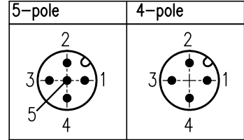
Contact arrangement
