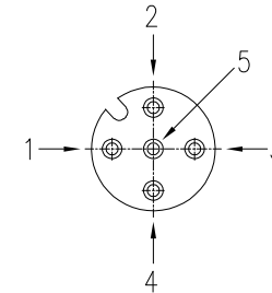
针位图 Contact arrangements
