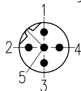
Contact arrangement
