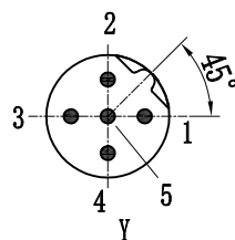
针位图 Contact arrangements
