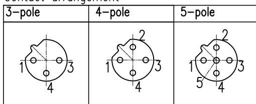
Contact arrangement
