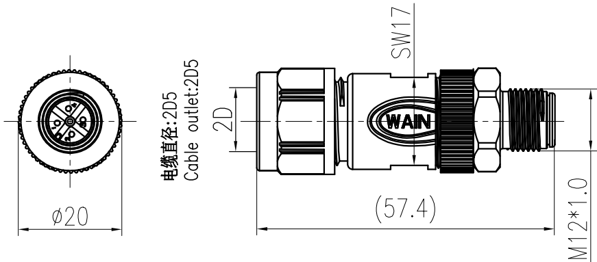
针位排布图 Contact arrangement
