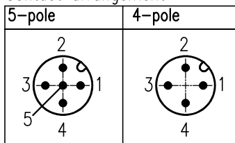
Contact arrangement
