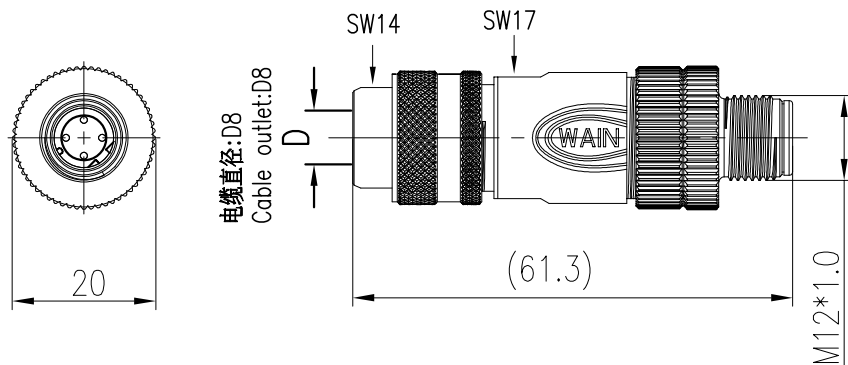
针位排布图 Contact arrangement
