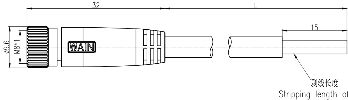
针位图 Contact arrangements
