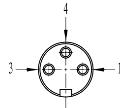
针位图 Contact arrangements
