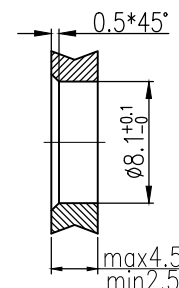
通孔安装 With bore hole
