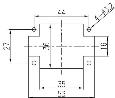
开孔尺寸图 (Panel cut out)
