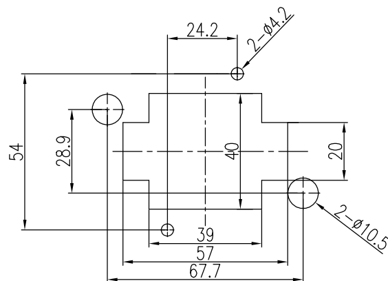
开孔尺寸图 (Panel cut out)
