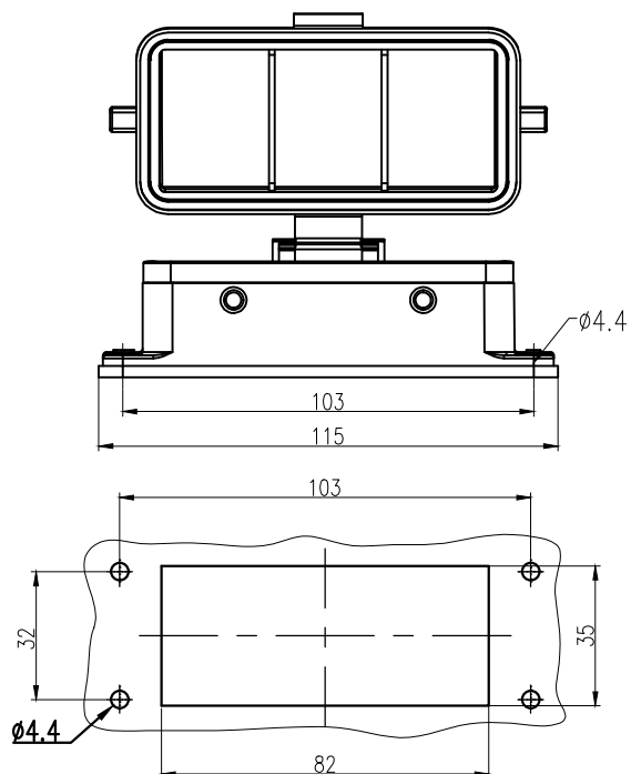
面板开孔图 Panel cut out
