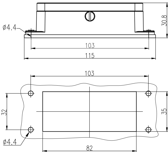
面板开孔图 Panel cut out
