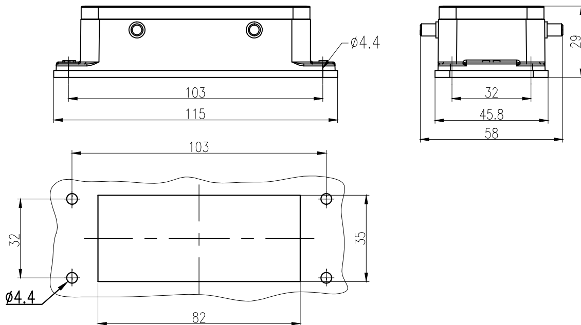
面板开孔图 panel cut out
