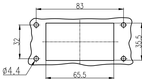
面板开孔图 Panel cut out
