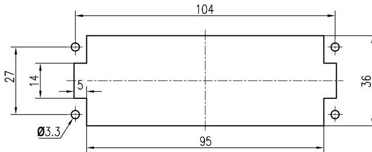
面板安装开孔图 Panel cut out
