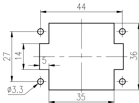
面板安装开孔图 Panel cut out
