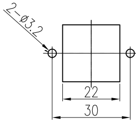
面板开孔图 Panel cut out
