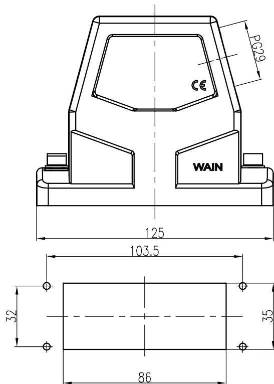
面板开孔图 Panel cut out
