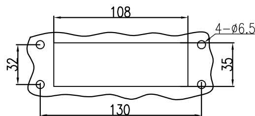
面板开孔图 Panel cut out
