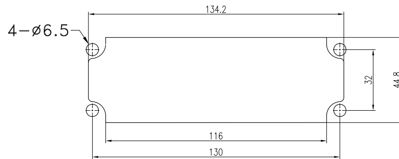
面板开孔图 Panel cut out
