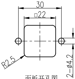
面板开孔图 Panel cut out
