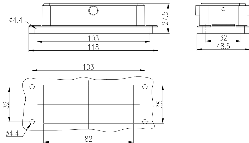
面板开孔图 Panel cut out
