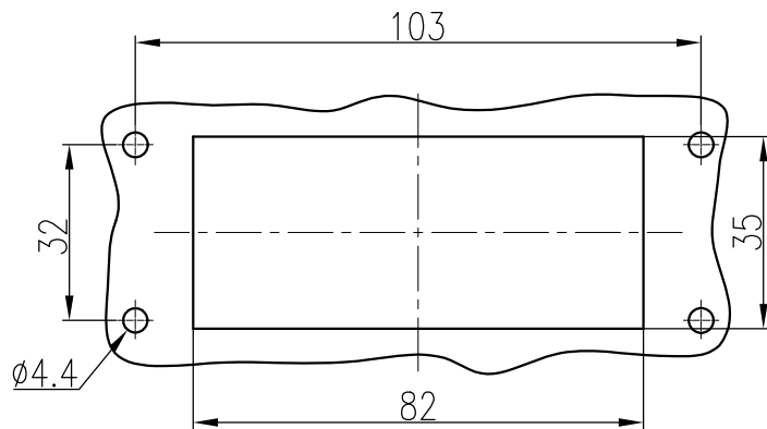
面板开孔图 Panel cut out
