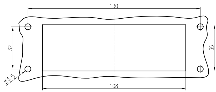
适用的面板开孔图 Applicable Panel cut out
