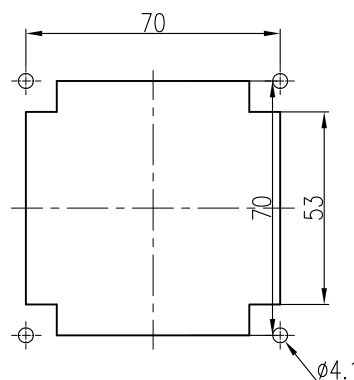
面板开孔图 Panel cut out
