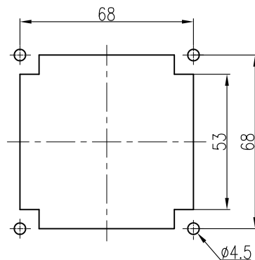
面板开孔图 Panel cut out
