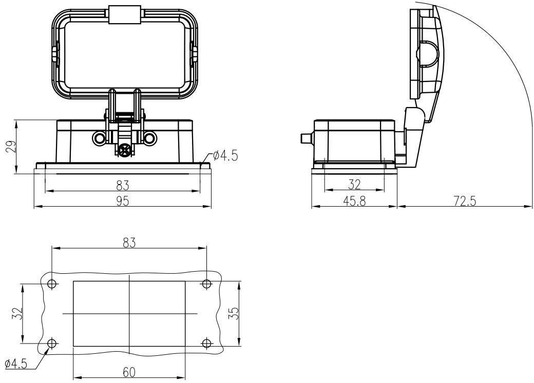
面板开孔图 Panel cut out
