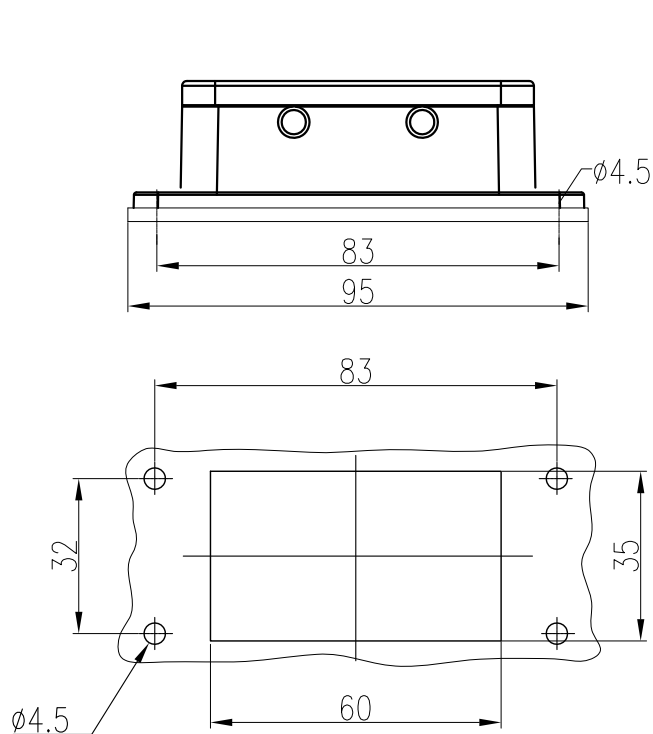
面板开孔图 Panel cut out
