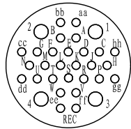
针位排布图 Contact arrangement
