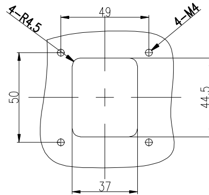
面板开孔图 Panel cut out
