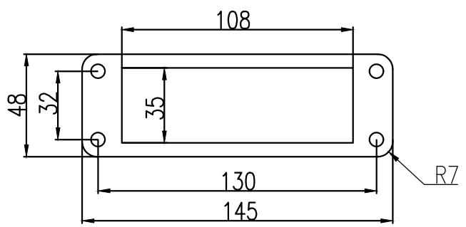
面板开孔图 Panel cut out
