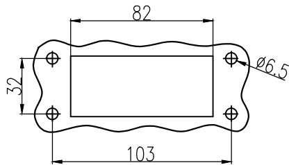
面板开孔图 Panel cut out
