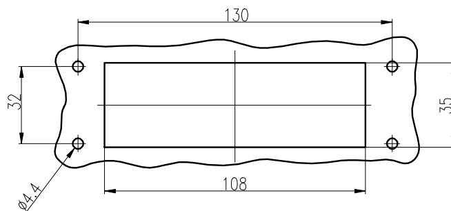
面板开孔图 Panel cut out
