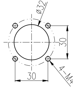
面板开孔图 Panel cut out
